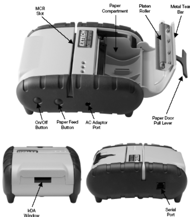
FIGURE 1: PRINTER OVERVIEW
