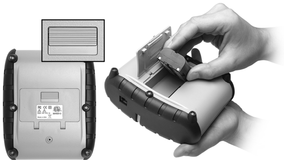
FIGURE 2: INSTALLING THE BATTERY CARTRIDGE
