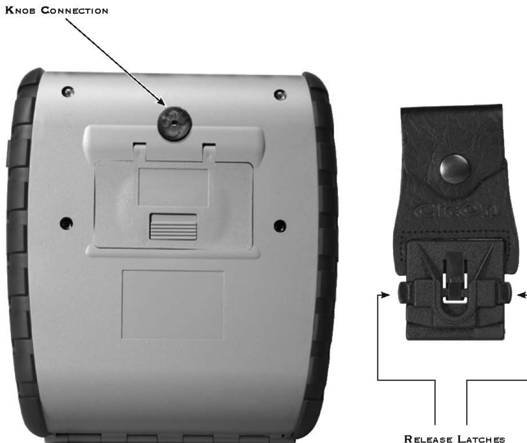
FIGURE 5: KNOB CONNECTION AND QUICK CLIP
